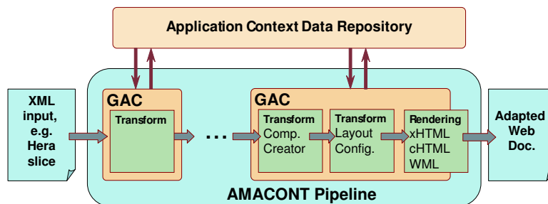
Fig. 3. Document Generation Pipeline.
